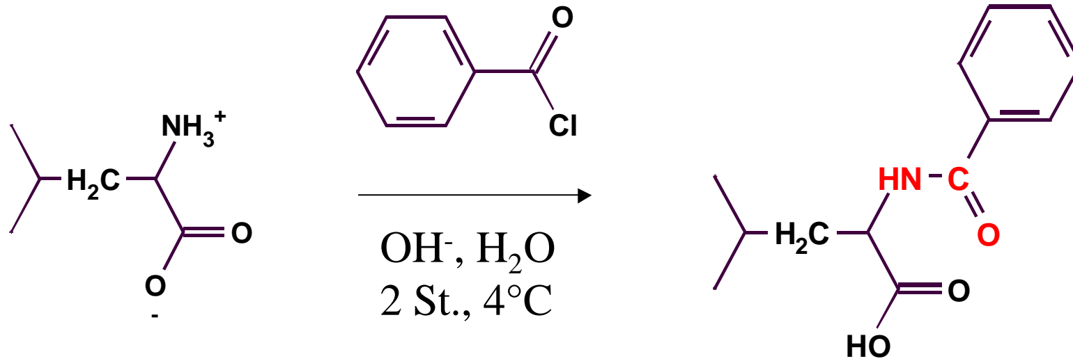
N-Benzoylvalin
